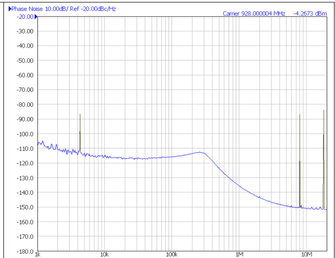
Figure 65. F2 (RX) Phase Noise and Spurs
