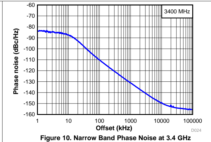
Figure 10. Narrow Band Phase Noise at 3.4 GHz
