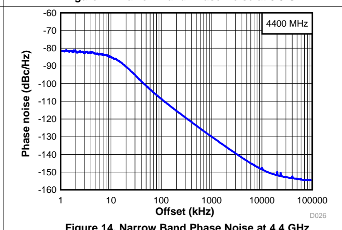
Figure 14. Narrow Band Phase Noise at 4.4 GHz
