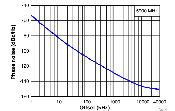
Figure 8. Open-Loop VCO Phase Noise at 5.9 GHz
