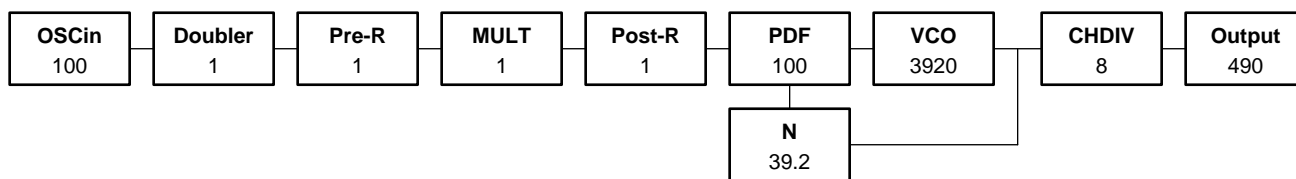
Figure 181. Application Example Frequency Plan
