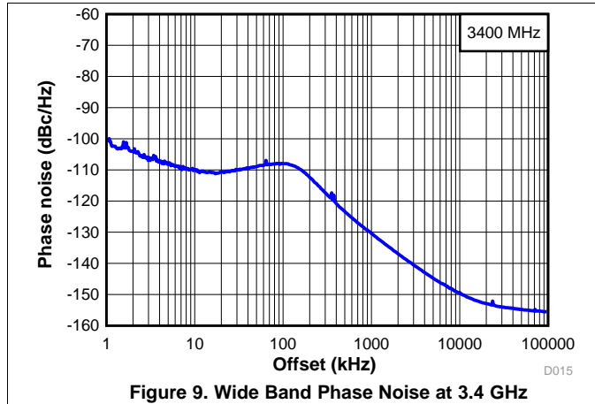
Figure 9. Wide Band Phase Noise at 3.4 GHz
