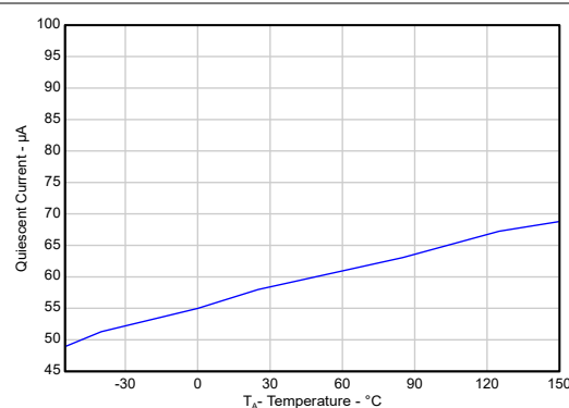
Figure 5-20. Quiescent Current vs Temperature ( I_L = 100\mu A ) (New Chip) V_{IN} = 6V , V_{OUT} = 5V
