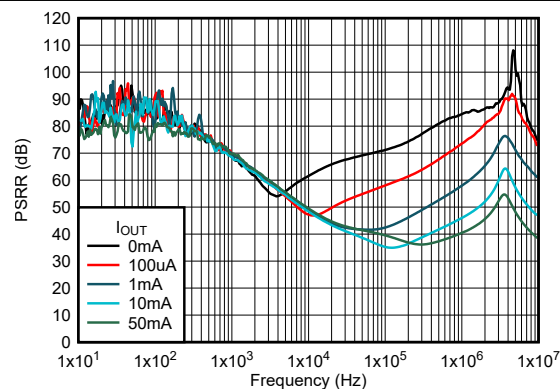
Figure 5-56. Ripple Rejection vs Frequency (Legacy Chip)
