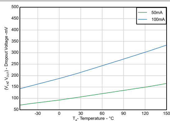
Figure 5-24. Dropout Voltage vs Temperature (New Chip) V_{IN} = 4.9V
