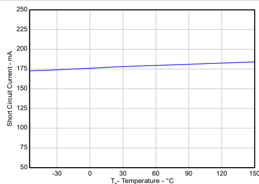
Figure 5-22. Short-Circuit Current vs Temperature (New Chip) V_{IN} = 6V , V_{OUT} = 0V
