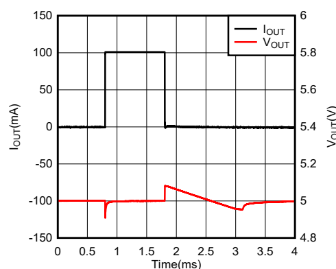
Figure 7-6. Load Transient Response vs Time (New Chip)
