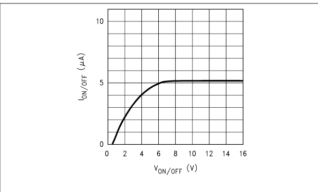
Figure 5-38. ON/OFF Pin Current vs V_{ON/OFF} (Legacy Chip)
