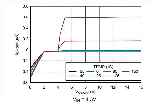
Figure 5-40. ON/OFF Pin Current vs V_{ON/OFF} (New Chip)
