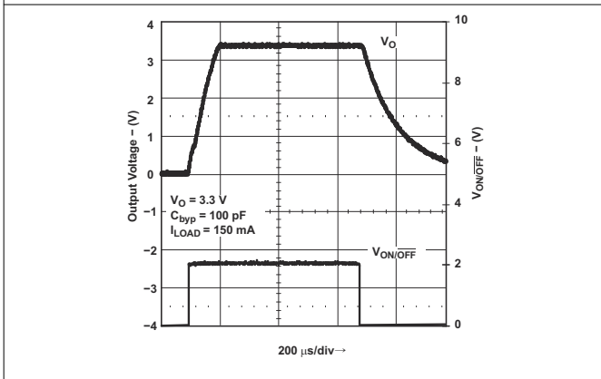
Figure 7-17. Turn-On Time for Legacy Chip
