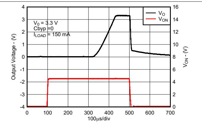
Figure 7-18. Turn-On Time for New Chip
