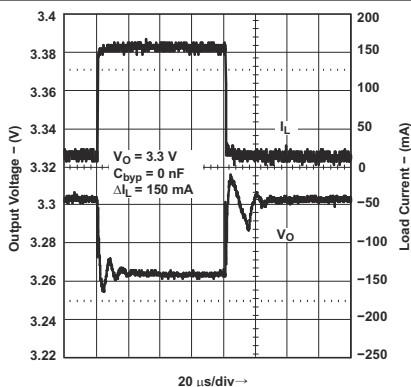
Figure 7-5. Load Transient Response for Legacy Chip
