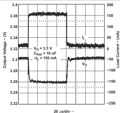
Figure 7-3. Load Transient Response for Legacy Chip
