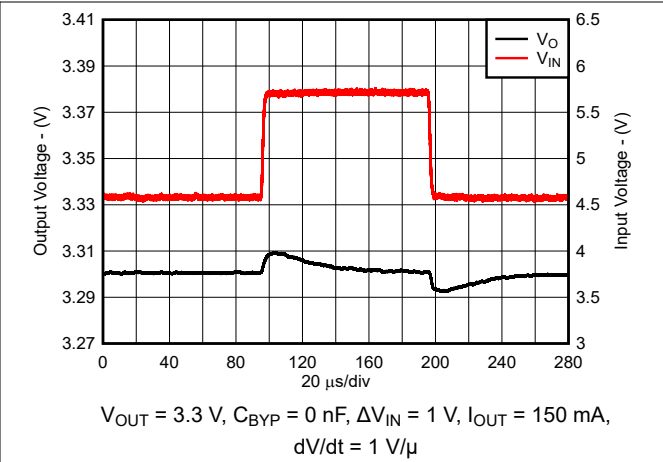
Figure 7-10. Line Transient Response for New Chip
