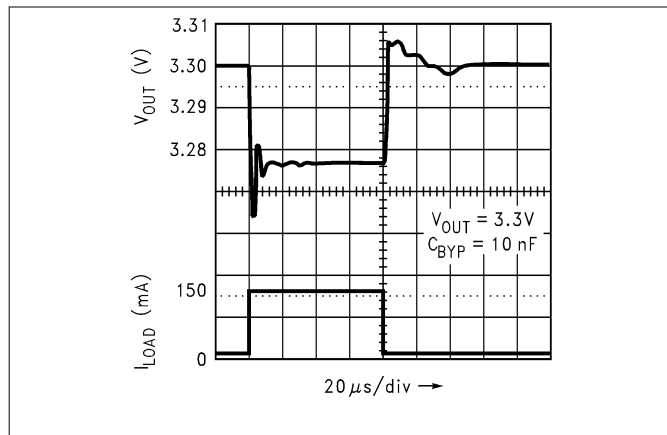
Figure 5-37. Load Transient Response (Legacy Chip)
