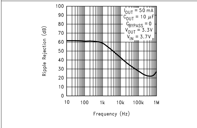
Figure 5-15. Ripple Rejection vs Frequency (Legacy Chip)
