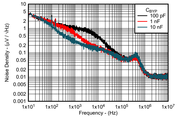
Figure 5-26. Output Noise Density vs Frequency (New Chip)
