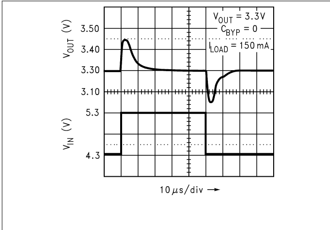
Figure 7-9. Line Transient Response for Legacy Chip
