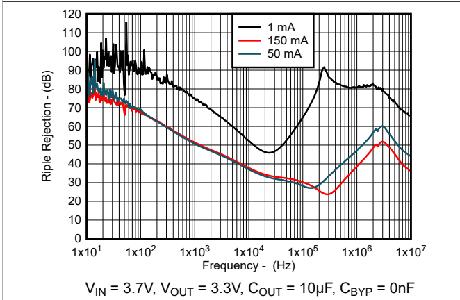
Figure 5-17. Ripple Rejection vs Frequency (New Chip)
