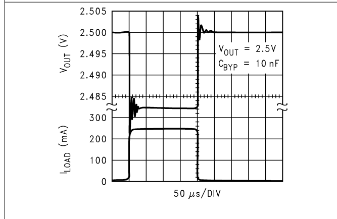
Figure 5-41. Load Transient Response (Legacy Chip)
