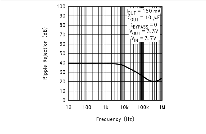
Figure 5-16. Ripple Rejection vs Frequency (Legacy Chip)
