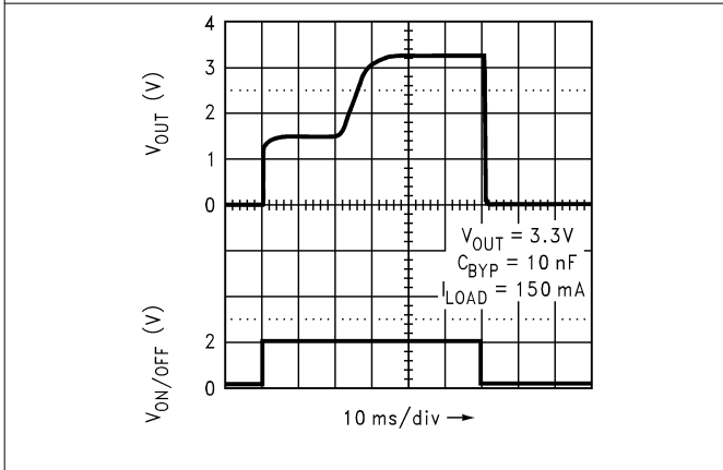
Figure 5-57. Turn-On Time (Legacy Chip)
