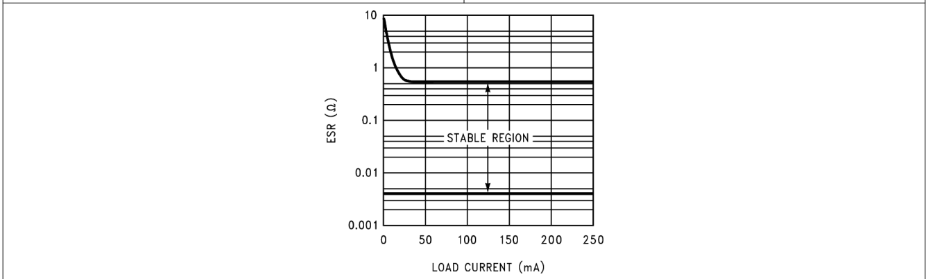
Figure 5-59. Stable ESR Range vs Load Current (Legacy Chip)
