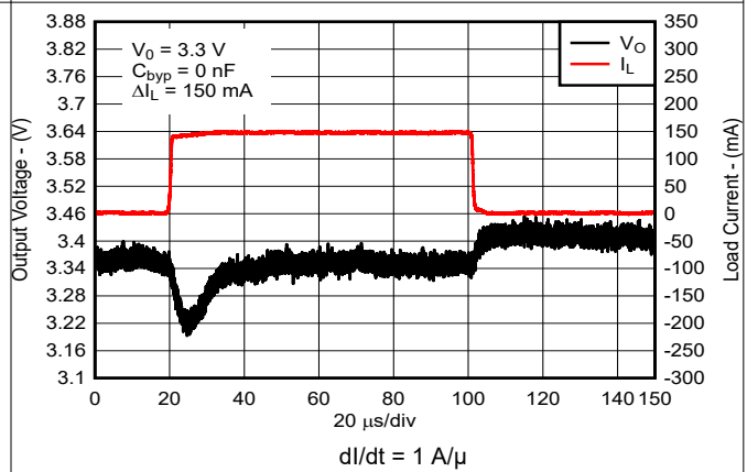
Figure 7-6. Load Transient Response for New Chip
