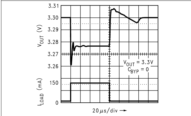
Figure 7-3. Load Transient Response for Legacy Chip
