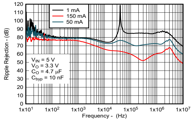
Figure 5-20. Ripple Rejection vs Frequency (New Chip)
