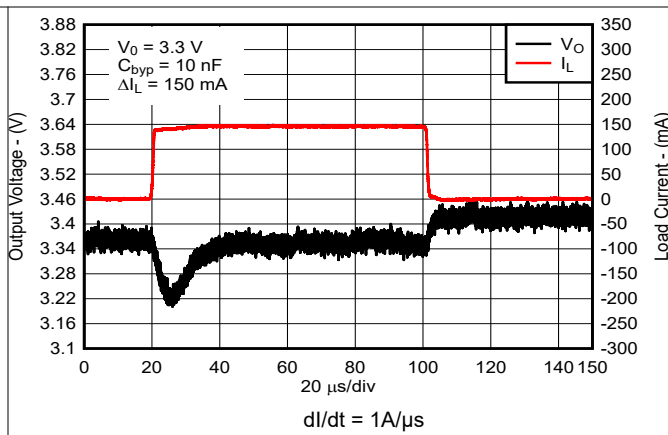
Figure 5-38. Load Transient (New Chip)
