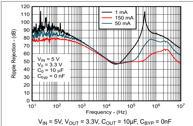
Figure 5-13. Ripple Rejection vs Frequency (New Chip)
