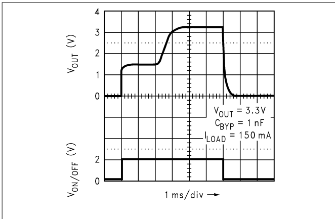
Figure 5-55. Turn-On Time (Legacy Chip)
