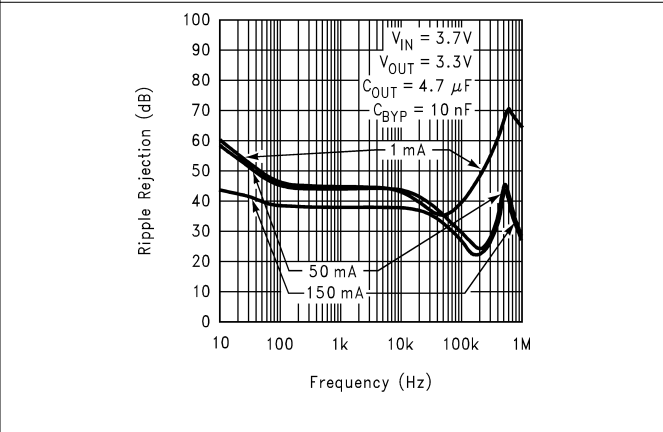
Figure 5-18. Ripple Rejection vs Frequency (Legacy Chip)
