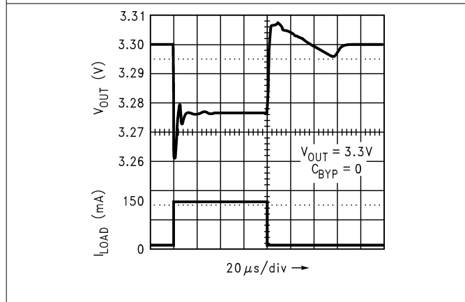
Figure 5-39. Load Transient Response (Legacy Chip)
