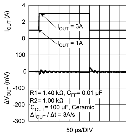
Figure 26. Load Transient Response
