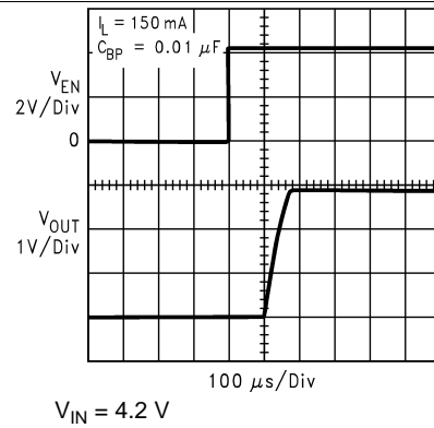
Figure 34. Enable Response
