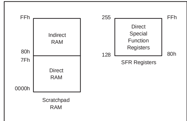
Figure 20. Register Map
