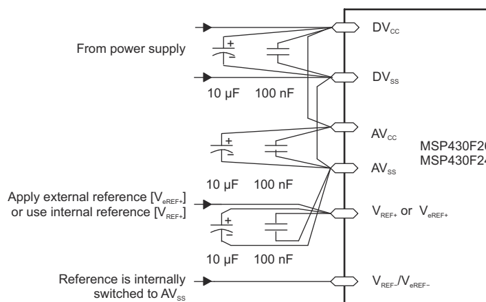
Figure 8-40. Supply Voltage and Reference Voltage Design V_{REF}/V_{REF-} = AV_{SS} , Internally Connected
