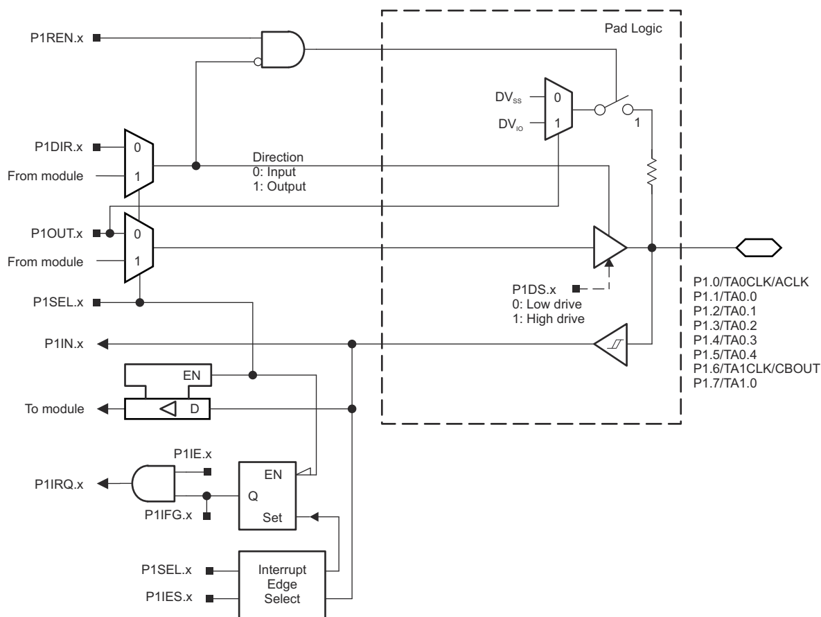
Figure 9-2. Port P1 (P1.0 to P1.7) Diagram
