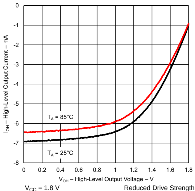
Figure 5-6. High-Level Output Current vs High-Level Output Voltage
