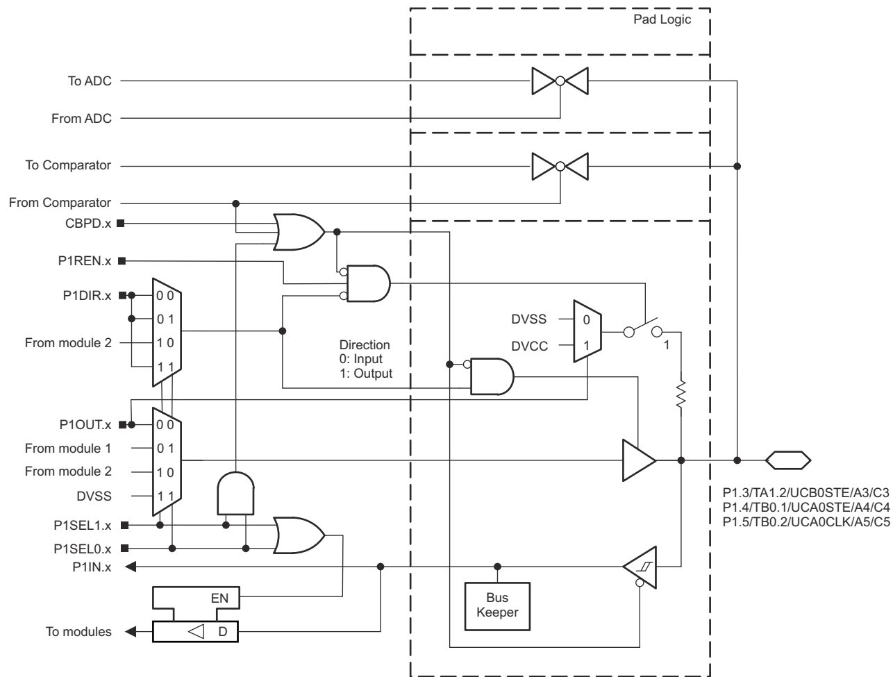
Figure 9-4. Port P1 (P1.3 to P1.5) Diagram
