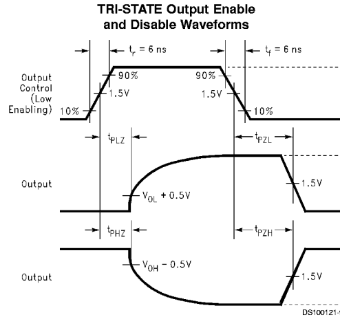
FIGURE 4. Switching Characteristic Measurement Waveforms
