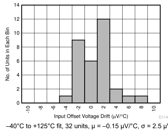
Figure 6-59. Input Offset Voltage Drift Distribution
