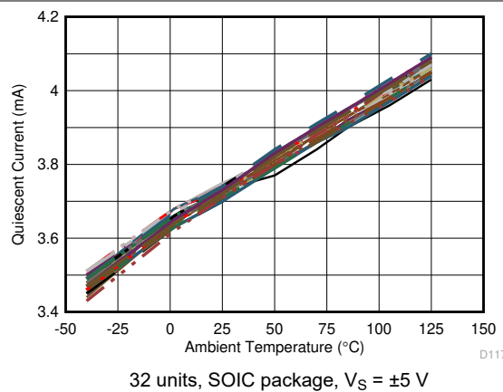
Figure 6-55. Quiescent Current vs Ambient Temperature
