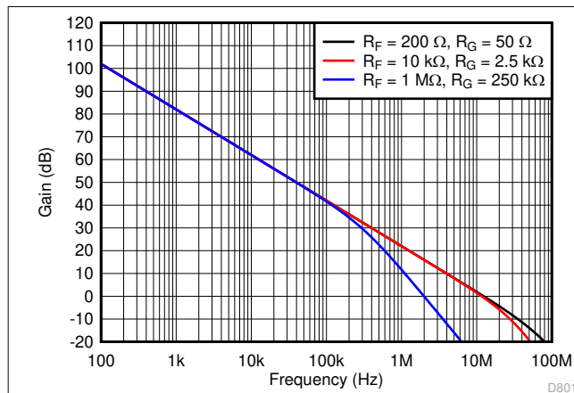
Figure 8-6. Loop-Gain vs Frequency for Circuit of Figure 8-5
