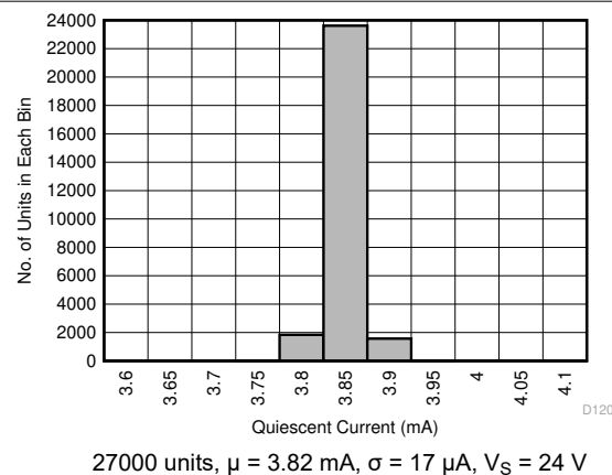
Figure 6-57. Quiescent Current Distribution
