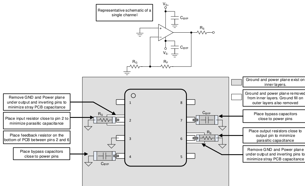
Figure 8-19. Layout Recommendation
