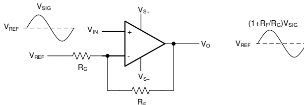
Figure 8-1. Noninverting Amplifier
