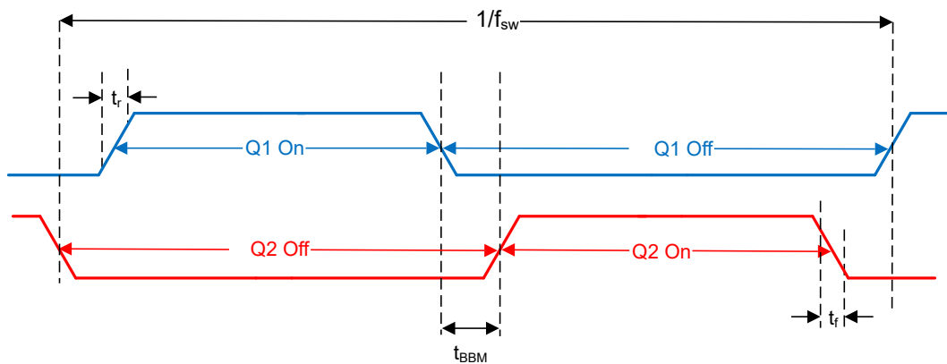
Figure 7-2. Timing Diagram
