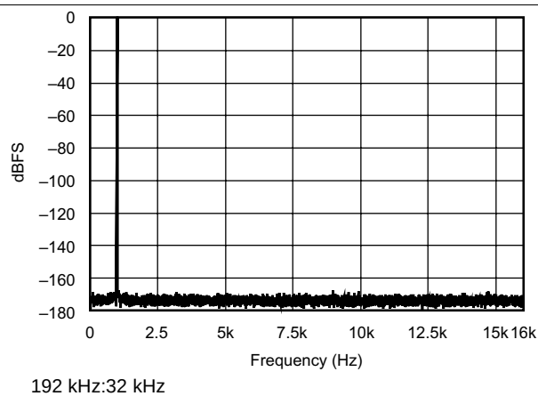
Figure 23. FFT With 1-kHz Input Tone at 0 dBFS
