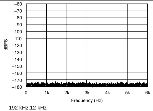
Figure 22. FFT With 1-kHz Input Tone at -60 dBFS
