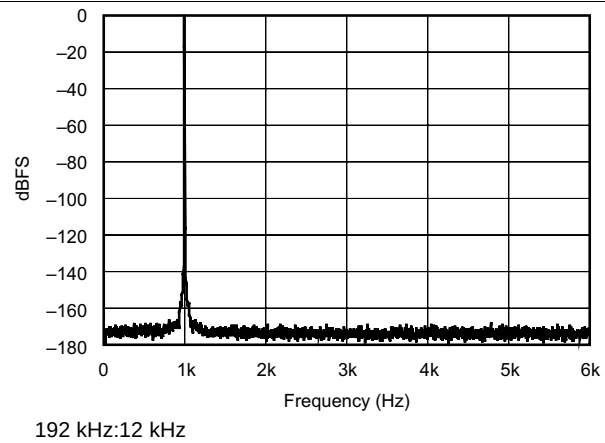
Figure 21. FFT With 1-kHz Input Tone at 0 dBFS
