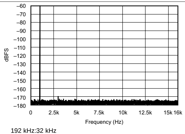
Figure 24. FFT With 1-kHz Input Tone at -60 dBFS
