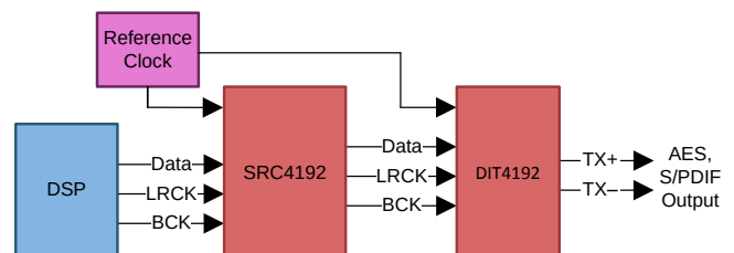
Simplified Application Diagram
