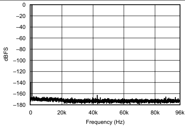
Figure 9. FFT With 1-kHz Input Tone at 0 dBFS
