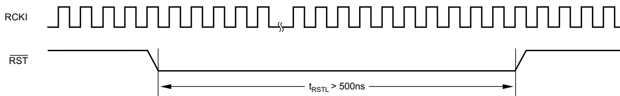
Figure 65. Reset Pulse Width Requirement
