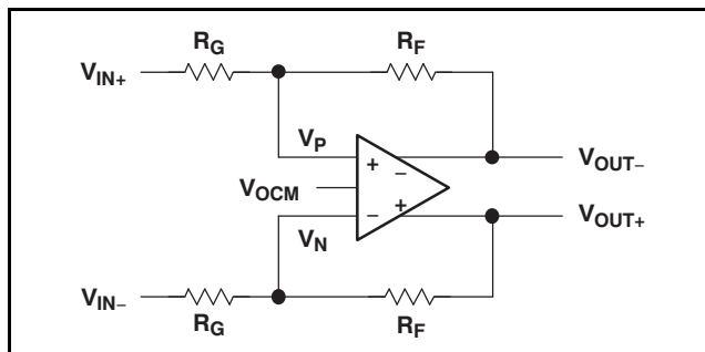
Figure 100. Diagram For Input Common-Mode Range Equations
