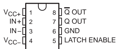
D AND PW PACKAGE (TOP VIEW)
