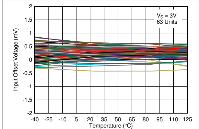
Figure 5-15. Input Offset Voltage vs. Temperature at 3V
