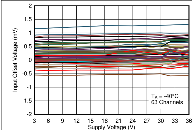
Figure 5-11. Input Offset Voltage vs. Supply Voltage at -40°C
