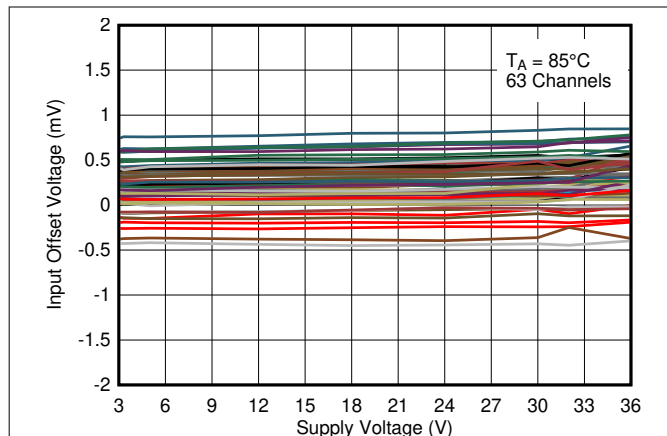
Figure 5-13. Input Offset Voltage vs. Supply Voltage at 85°C
