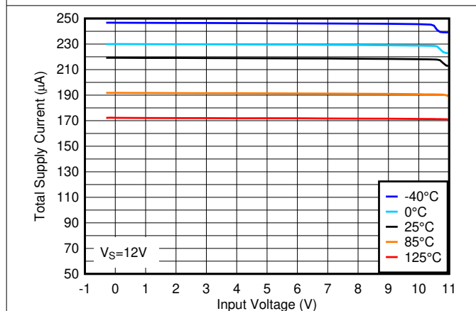
Figure 5-5. Total Supply Current vs. Input Voltage at 12V
