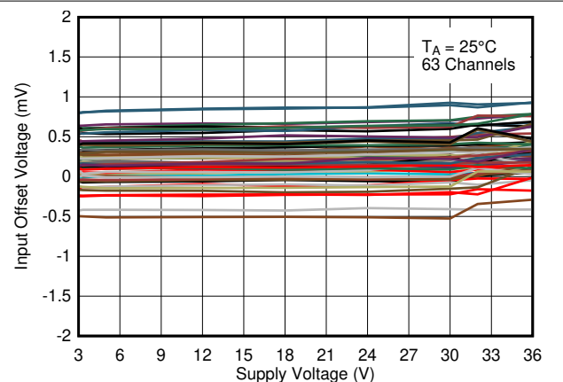
Figure 5-12. Input Offset Voltage vs. Supply Voltage at 25°C
