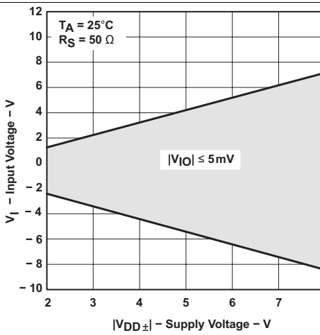
Figure 12. Input Voltage vs Supply Voltage
