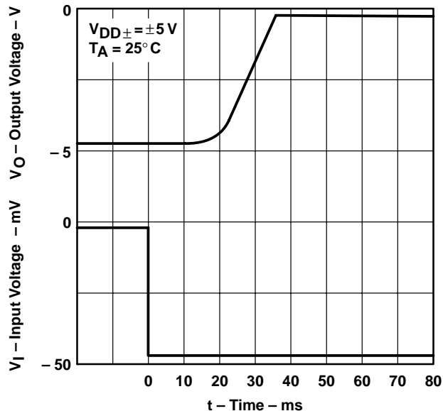
Figure 34. Overload Recovery
