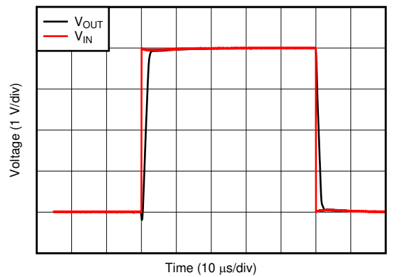
Figure 7-28. Overload Recovery
