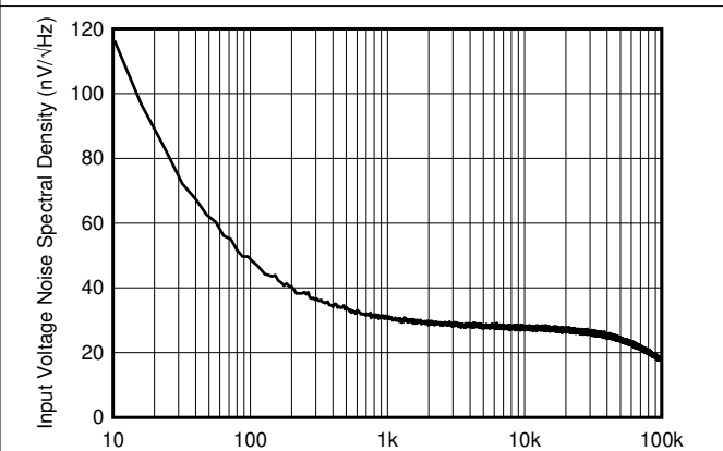
Figure 7-18. Input Voltage Noise Spectral Density
