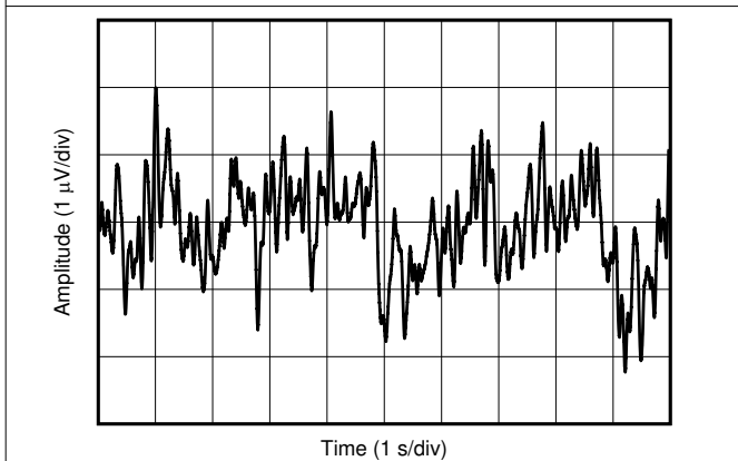
Figure 7-17. 0.1 Hz to 10 Hz Integrated Voltage Noise
