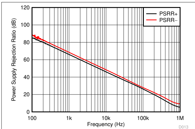
Figure 7-13. PSRR vs Frequency
