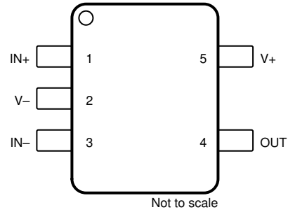
Figure 4-2. TLV9361-Q1 DCK Package 5-Pin SC70 (Top View)
