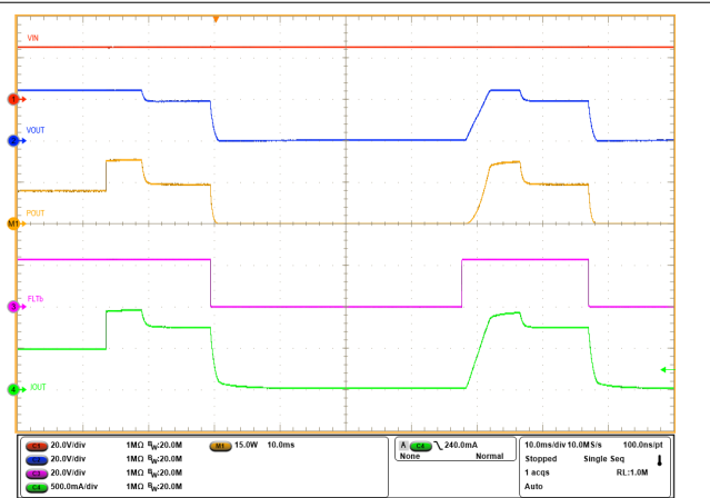
Figure 9-5. 15-W Power Limiting with TPS16410 ( I_{OUT} < I_{OCP} )
