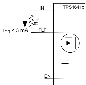
Figure 8-16. \overline{\text{FLT}} Output in the TPS1641x
