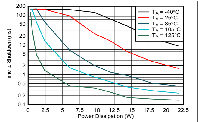
Figure 7-14. Thermal Shutdown Time vs Power Dissipation with V_{IN} = 12\text{ V}
