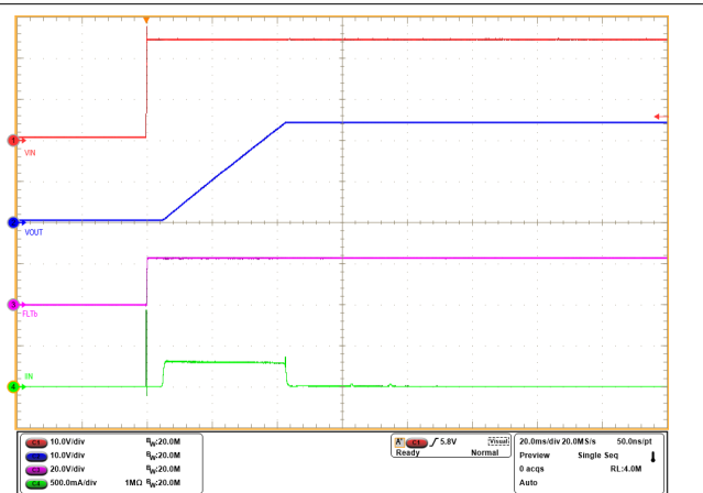
Figure 9-3. Inrush Current Control for Hot Plug-in at Input
