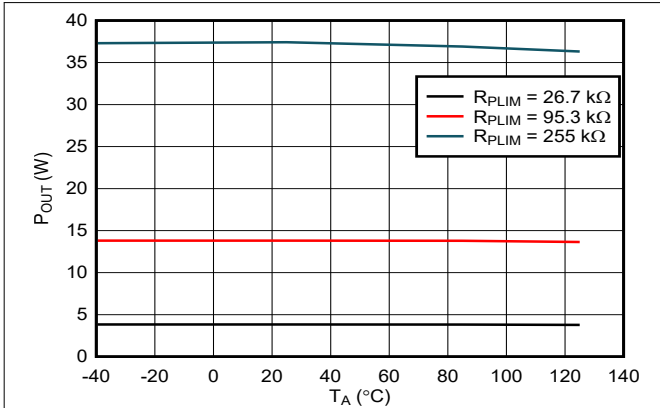
Figure 7-13. Output Power Limit vs Temperature for TPS16410 and TPS16411 with V_{IN} = 24\text{ V}
