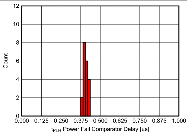
Figure 7-26. PFI to PFO (t PLH ) Delay Histogram for TPS3705-33 Devices at 125°C (Unit Count = 20)
