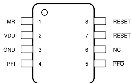
Figure 6-2. TPS3707-xx D Package 8-Pin SOIC Top View
