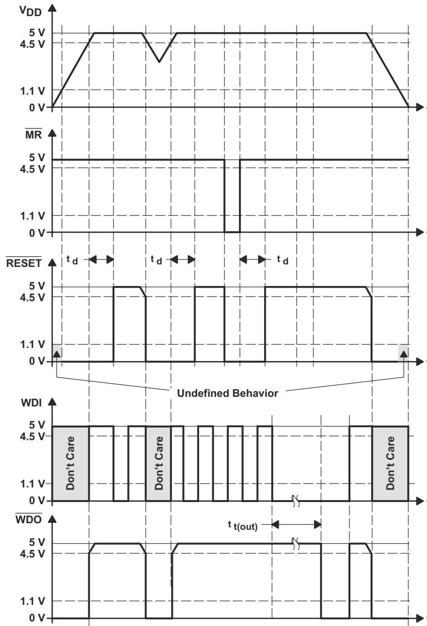
Figure 7-1. Timing Diagrams
