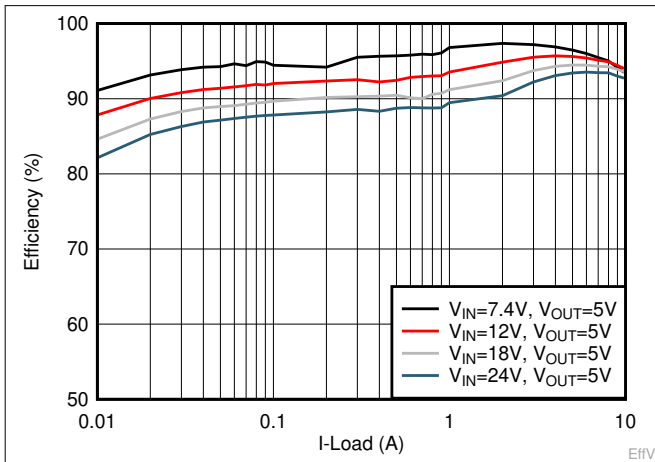
Figure 8-2. Efficiency Curve
