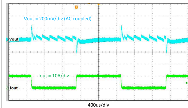
Figure 8-16. Transient Response, 0 A to 10 A, Slew Rate = 2.5 A/µs
