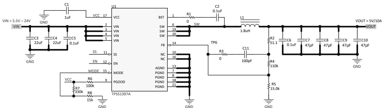
Figure 8-1. 5-V, 10-A Reference Design
