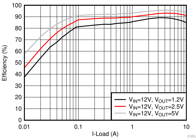
Figure 6-17. Efficiency vs Load Current, F SW = 500 kHz, OOA
