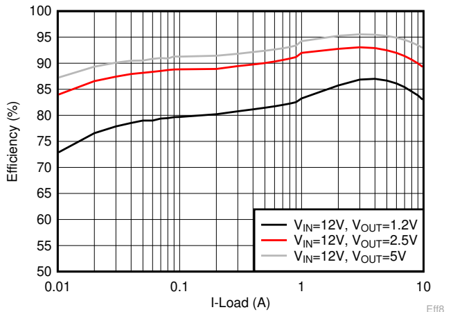
Figure 6-16. Efficiency vs Load Current, F SW = 800 kHz, Eco-mode
