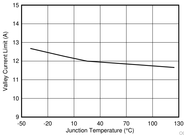
Figure 6-11. Valley Current Limit vs Junction Temperature
