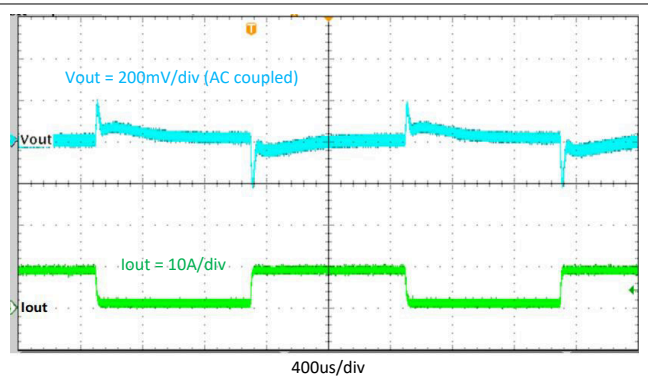
Figure 8-15. Transient Response, 1 A to 9 A, Slew Rate = 2.5 A/µs
