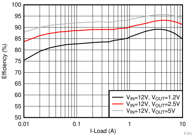
Figure 6-15. Efficiency vs Load Current, F SW = 500 kHz, Eco-mode
