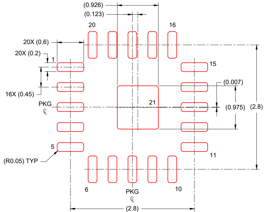
SOLDER PASTE EXAMPLE BASED ON 0.1 mm THICK STENCIL PRINTED SOLDER COVERAGE BY AREA UNDER PACKAGE SCALE: 20X
