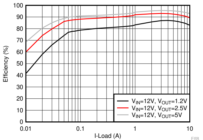
Figure 6-18. Efficiency vs Load Current, F SW = 800 kHz, OOA
