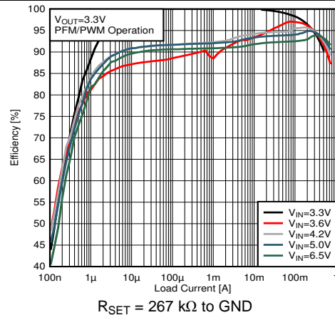
Figure 19. Efficiency Power Save Mode V_{OUT} = 3.3\text{ V}
