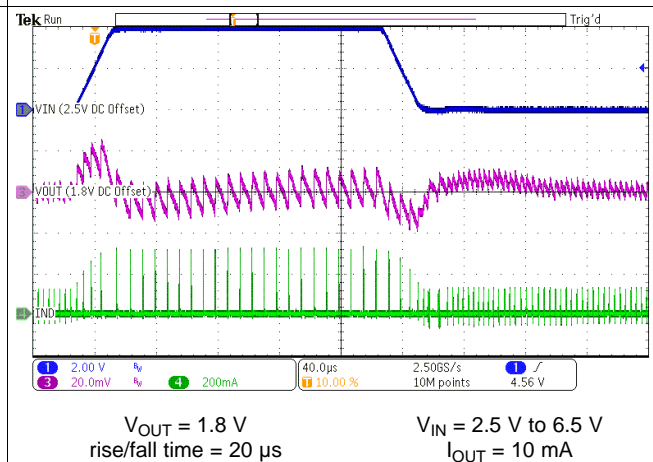
Figure 47. Line Transient PFM Mode
