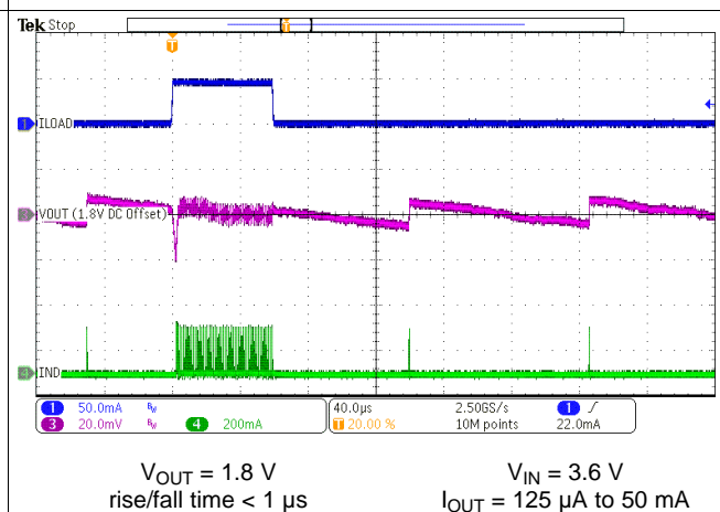
Figure 49. Load Transient PFM Mode
