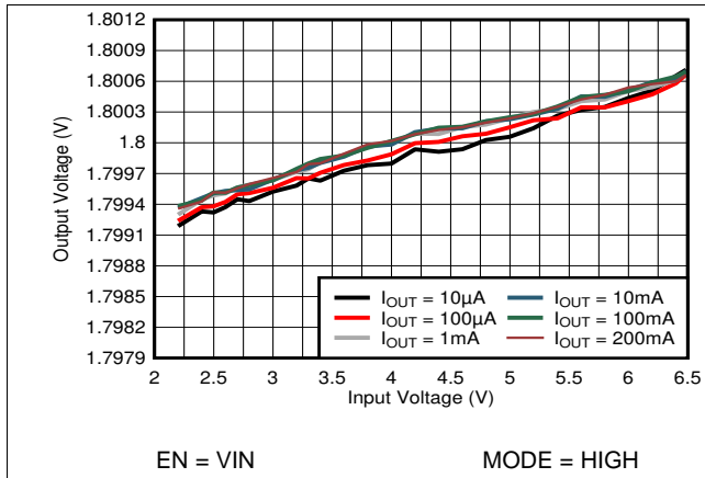
Figure 44. Output Voltage Accuracy (Line Regulation)
