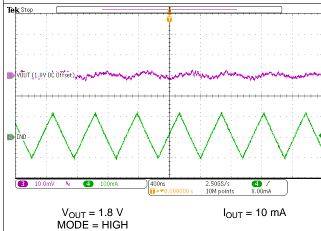
Figure 46. Output Voltage Ripple, PWM Operation
