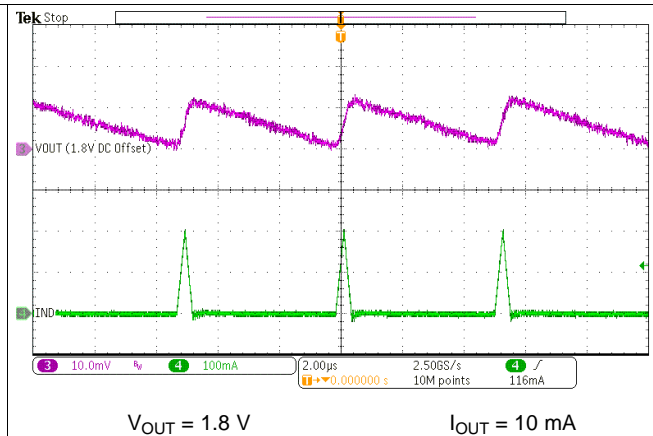
Figure 45. Output Voltage Ripple, PFM Operation
