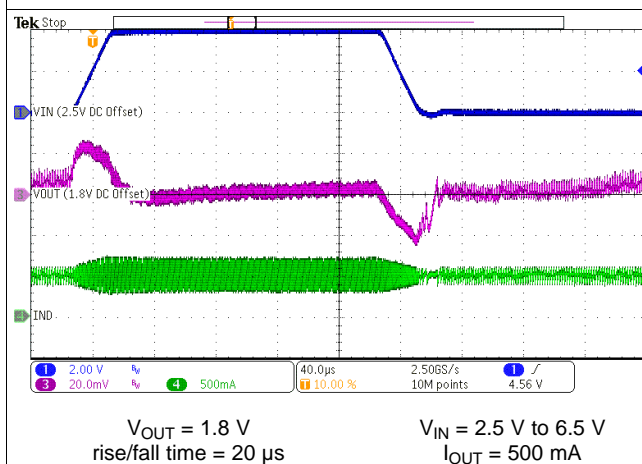
Figure 48. Line Transient PWM Mode
