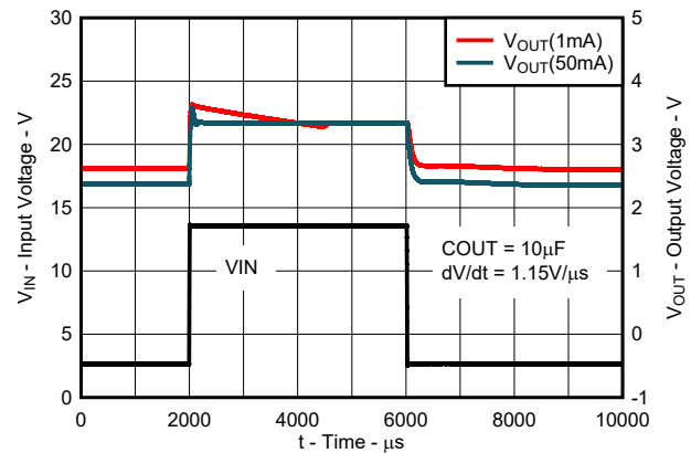
Figure 8-11. Fast Line Transient Response for New Chip
