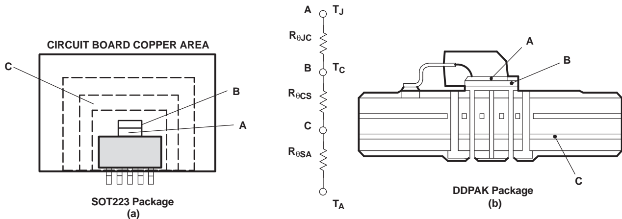
Figure 19. Thermal Resistances
