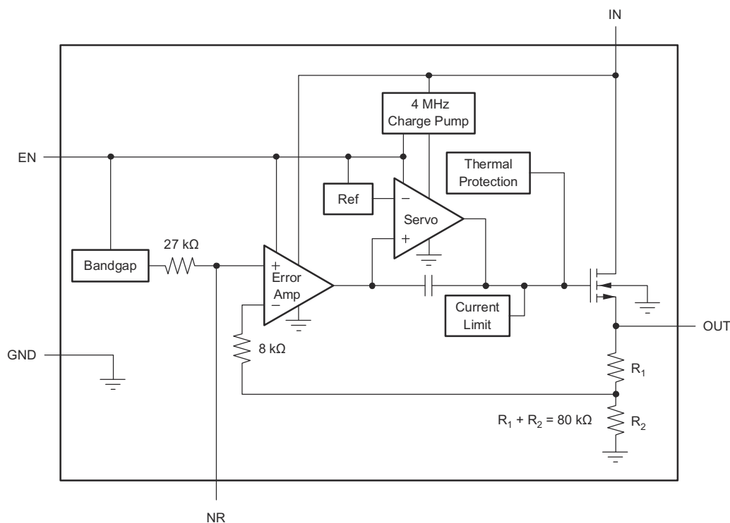
Figure 6-1. Fixed-Voltage Version
