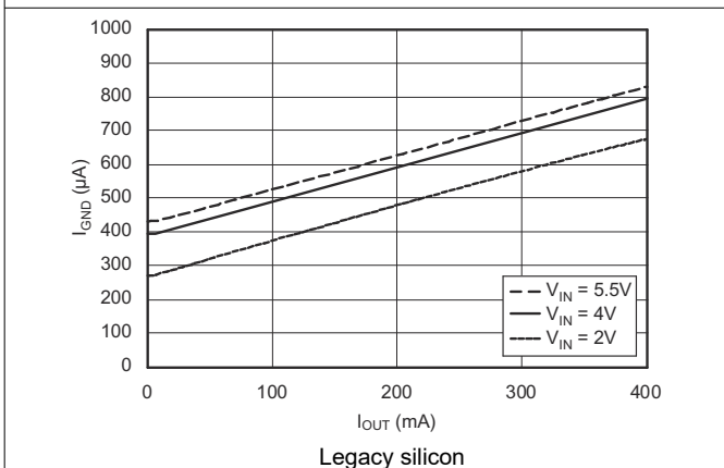
Figure 5-11. Ground Pin Current vs Output Current
