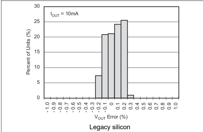
Figure 5-9. Output Voltage Accuracy Histogram
