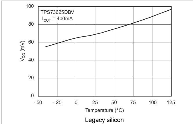
Figure 5-7. Dropout Voltage vs Temperature
