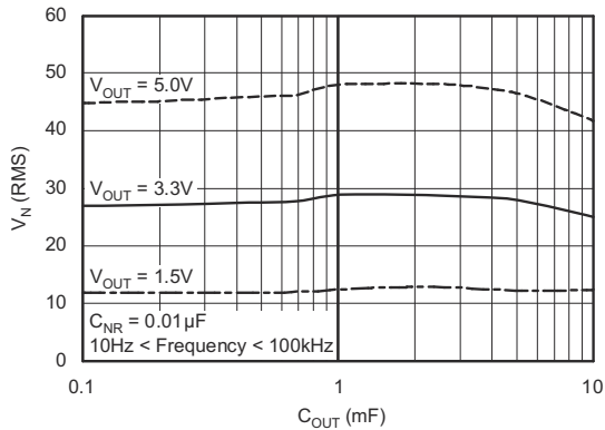
Figure 5-31. RMS Noise Voltage vs C_{OUT} Legacy silicon
