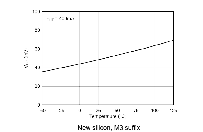
Figure 5-8. Dropout Voltage vs Temperature
