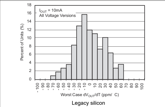
Figure 5-10. Output Voltage Drift Histogram
