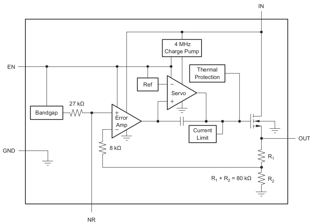
Figure 6-1. Fixed-Voltage Version
