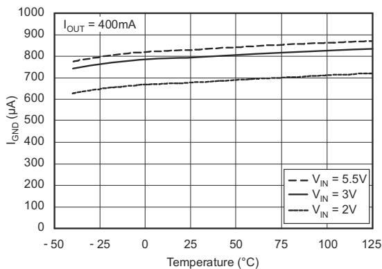
Figure 5-13. Ground Pin Current vs Temperature
