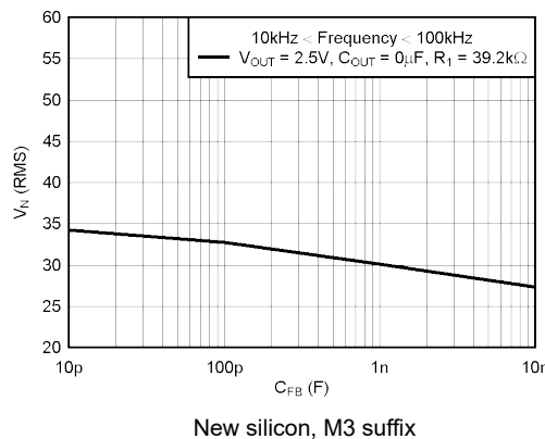
Figure 5-48. TPS73601 RMS Noise Voltage vs CFB
