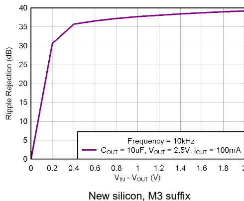
Figure 5-26. PSRR (Ripple Rejection) vs V_{IN} - V_{OUT}
