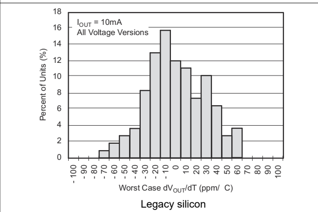
Figure 5-10. Output Voltage Drift Histogram
