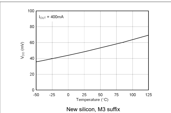
Figure 5-8. Dropout Voltage vs Temperature
