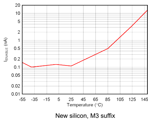
Figure 5-46. IENABLE vs Temperature
