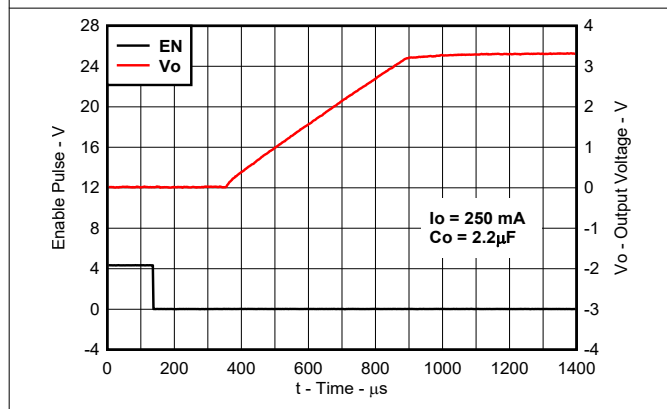
Figure 5-42. TPS76633 Output Voltage vs Time (New Chip)
