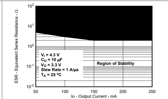
Figure 5-54. Typical Region of Stability ESR vs Output Current (New Chip)
