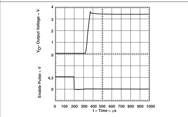
Figure 5-41. TPS76633 Output Voltage vs Time (Legacy Chip)
