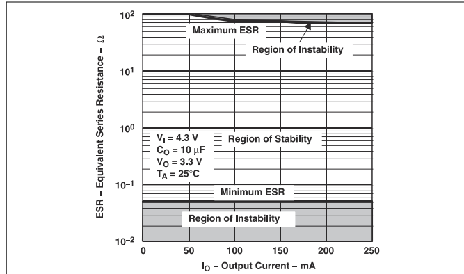
Figure 5-53. Typical Region of Stability ESR vs Output Current (Legacy Chip)
