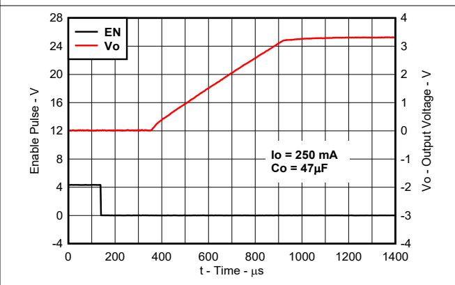
Figure 5-43. TPS76633 Output Voltage vs Time (New Chip)
