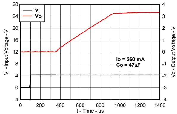
Figure 5-45. TPS76633 Output Voltage vs Time (New Chip)
