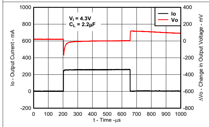
Figure 5-40. TPS76633 Load Transient Response (New Chip)
