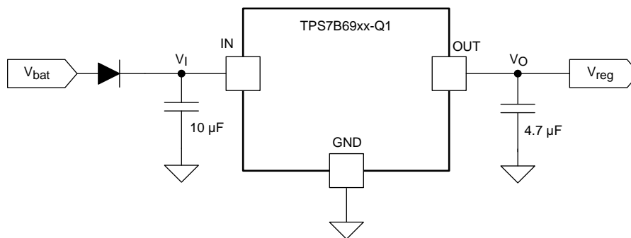
Figure 25. Typical Application Schematic for TPS7B69xx-Q1
