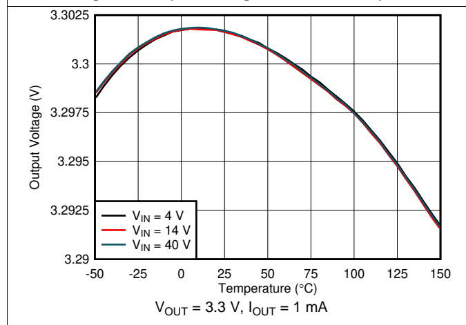
Figure 9. Output Voltage vs Ambient Temperature
