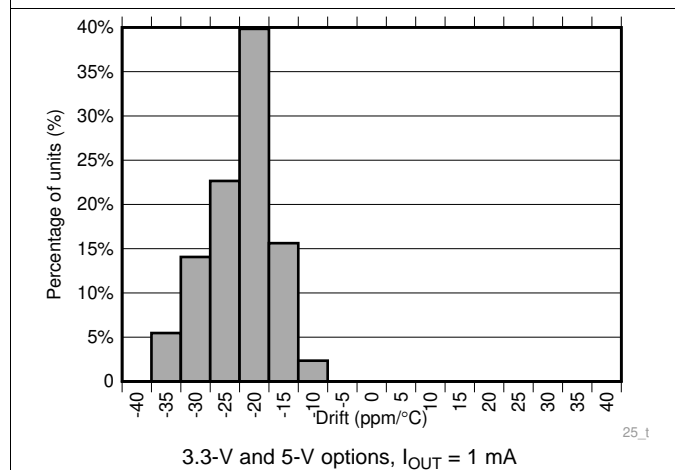
Figure 11. Temperature Drift Histogram (25°C to 150°C)
