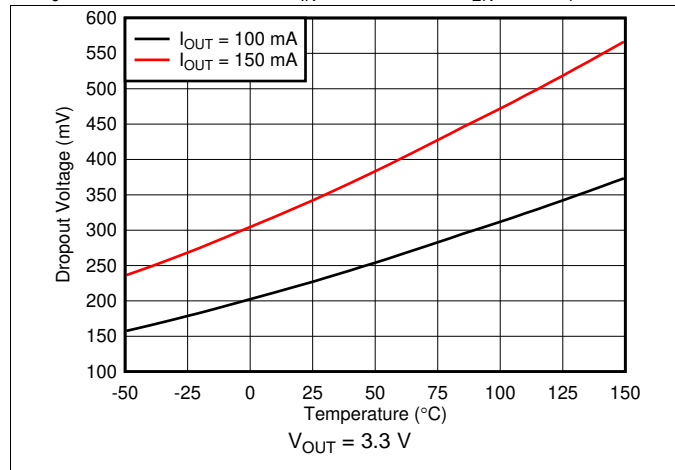
Figure 7. Dropout Voltage vs Ambient Temperature
