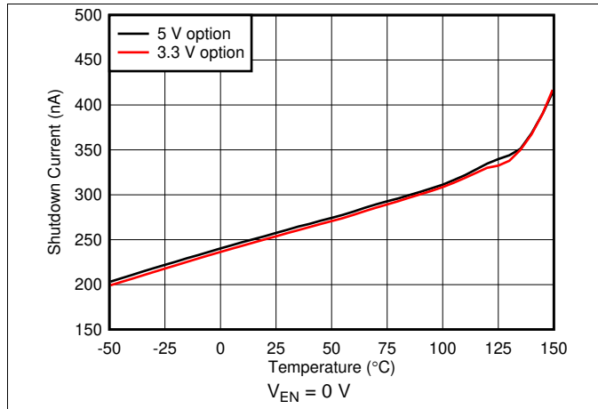
Figure 1. Shutdown Current vs Ambient Temperature
