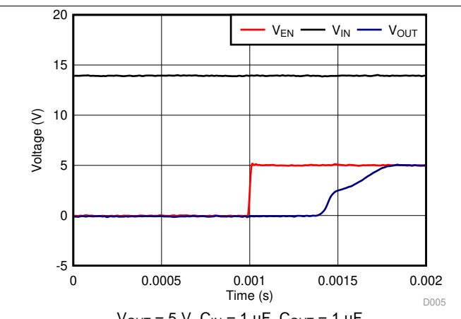
Figure 18. Startup With Enable
