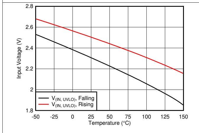
Figure 17. UVLO vs Ambient Temperature
