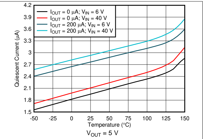
Figure 2. Quiescent Current vs Ambient Temperature
