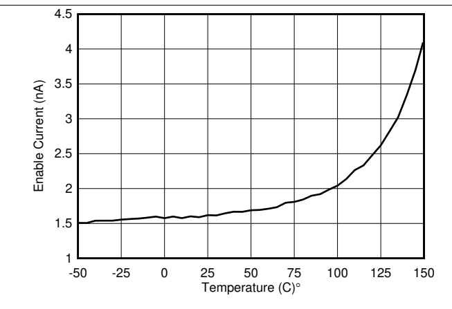
Figure 16. Enable Current vs Ambient Temperature
