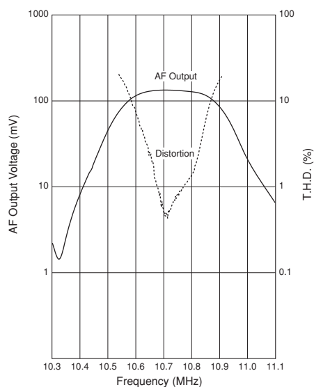
CDSCB10M7GA105A-R0
