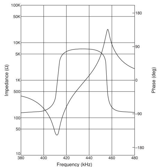
CDBLB455KCAY03-B0
