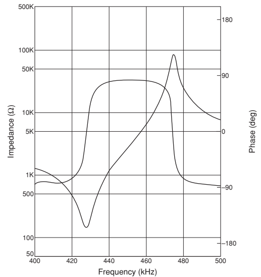
CDBLB455KCAX31-B0
