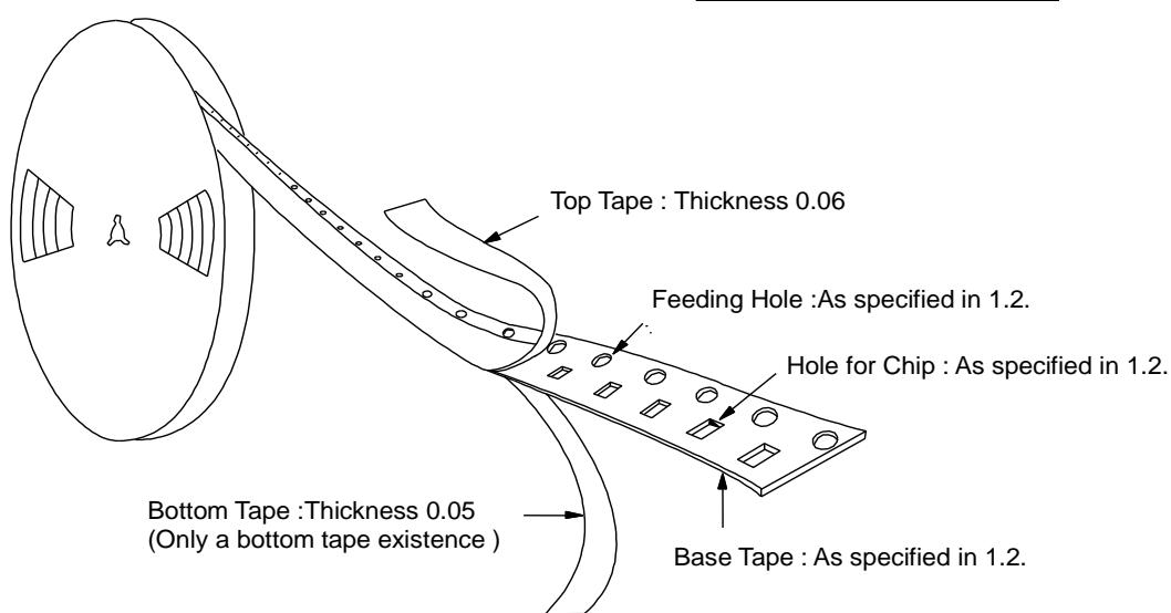
Fig.3 Taping Diagram
