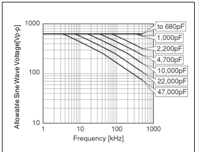
U2J(7U) Char. Rated Voltage : DC630V
