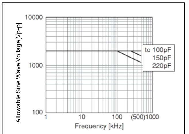
U2J(7U) Char. Rated Voltage : DC2 kV
