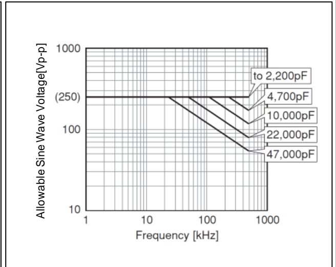
U2J(7U) Char. Rated Voltage : DC250V
