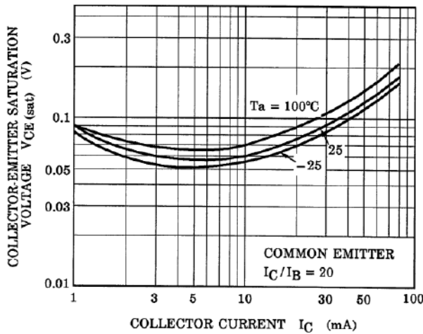
Fig. 10.21 RN1303 V_{CE(sat)}-I_C
