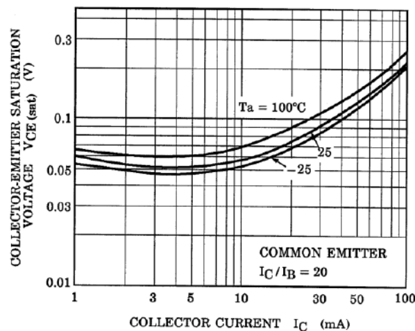
Fig. 10.23 RN1305 V_{CE(sat)}-I_C
