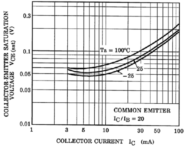
Fig. 10.20 RN1302 V_{CE(sat)}-I_C
