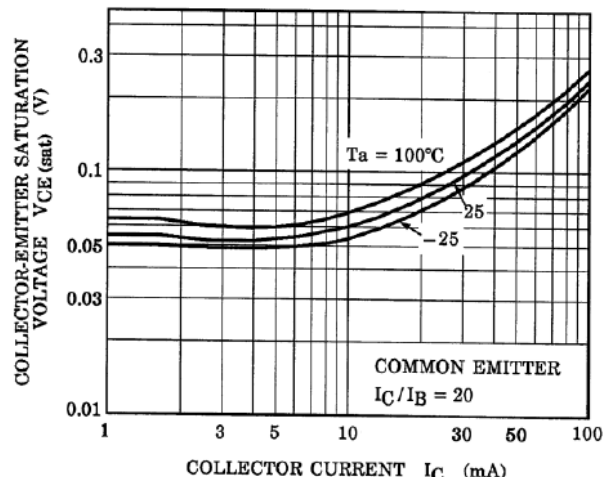
Fig. 10.24 RN1306 V_{CE(sat)}-I_C
