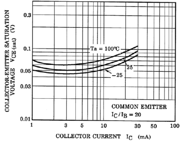
Fig. 10.22 RN1304 V_{CE(sat)}-I_C
