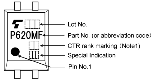
Marking example of TLP620MF
