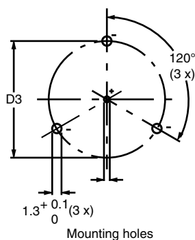
Mounting holes
