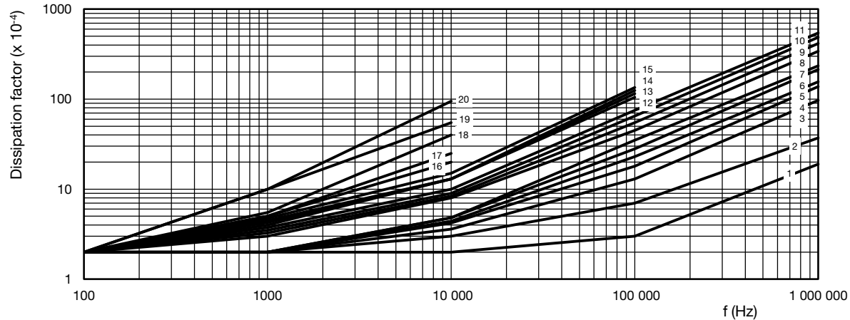
Tangent of loss angle as a function of frequency (typical curve)
