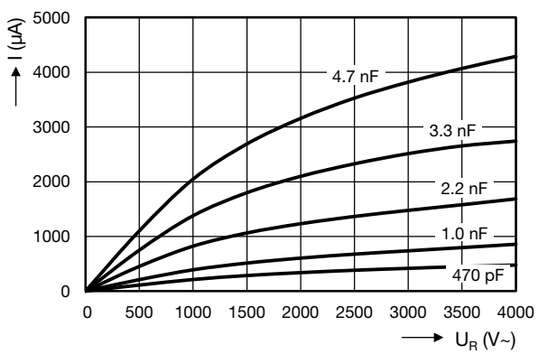
AC CURRENT VS. VOLTAGE (typical)
