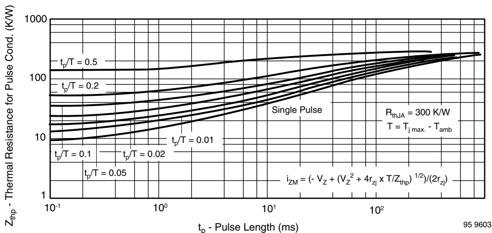
Fig. 11 - Thermal Response
