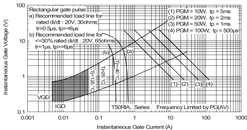
Fig. 8 - Gate Characteristics
