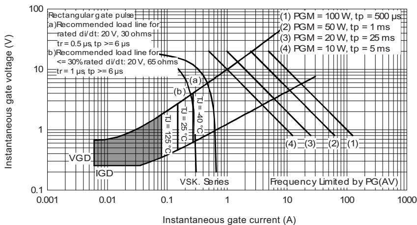
Fig. 12 - Gate Characteristics
