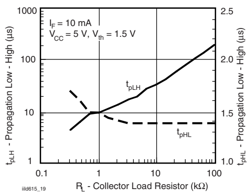
Fig. 19 - -4, Propagation Delay vs. Collector Load Resistor
