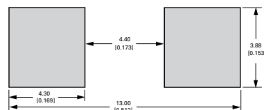
Recommended Pad Layout
