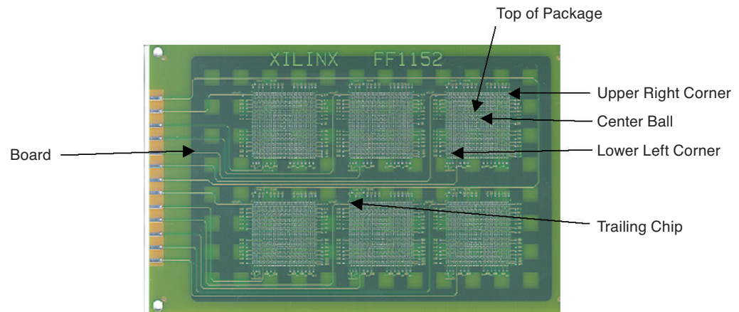
Figure 7-4: Temperature Measurement Locations
