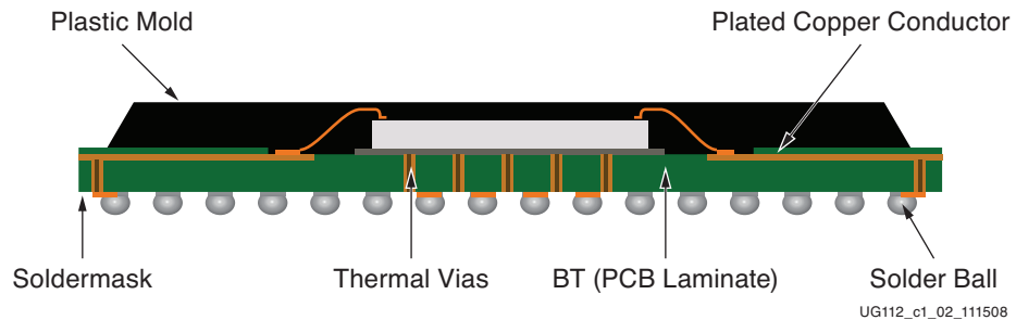
Figure 1-2: Cavity-Up Ball Grid Array Package
