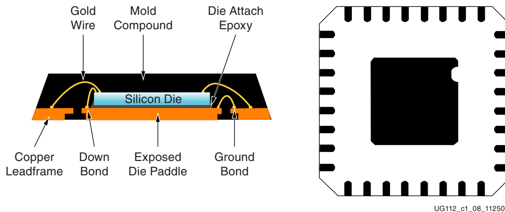
Figure 1-8: QFN Cross Section (Left) and Bottom View (Right)
