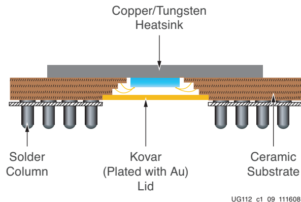
Figure 1-9: CG560 Package
